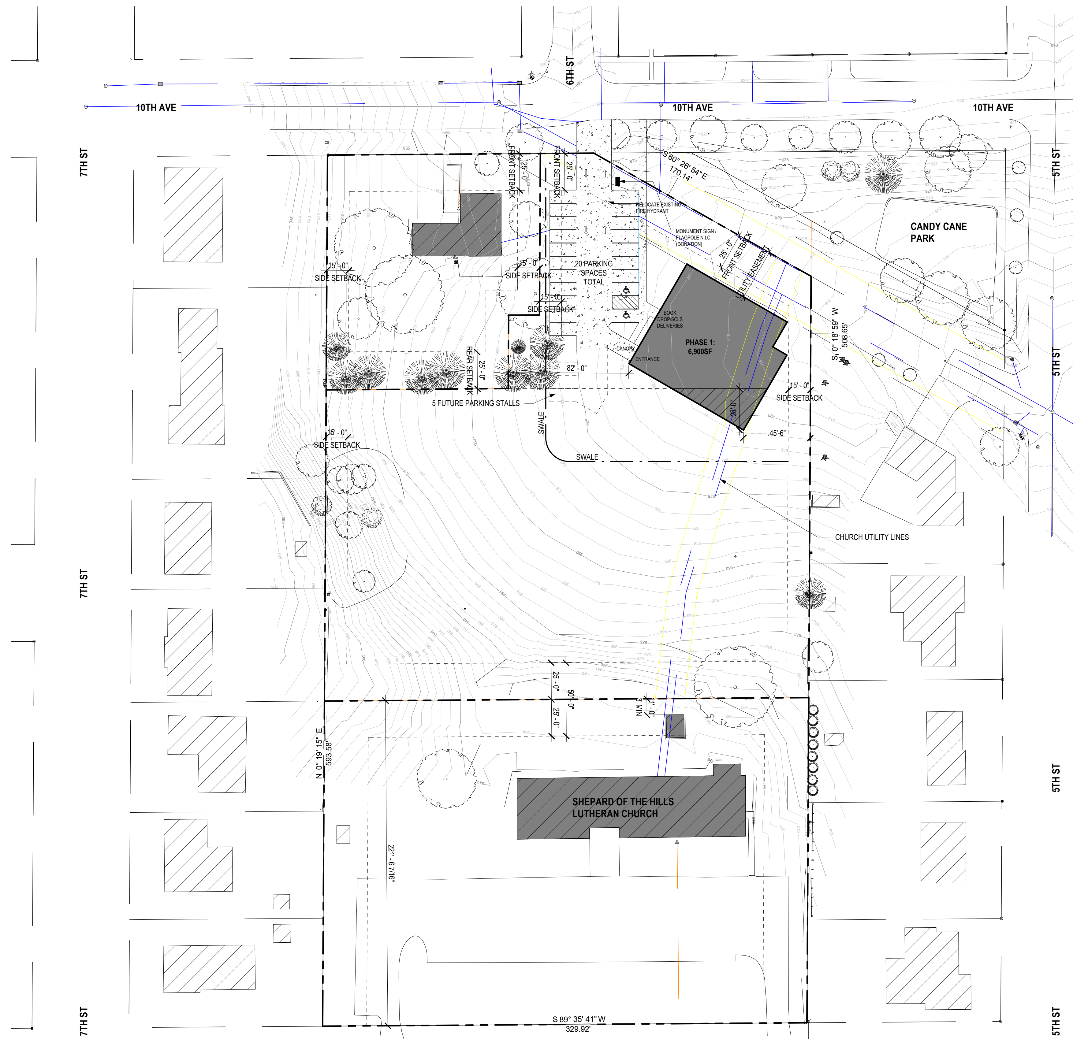
1 ARCHITECTURAL SITE PLAN-OPTION 4 1" = 40'-0"
